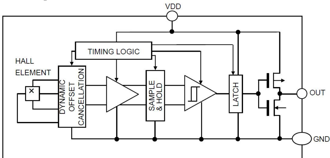
Figure 3, Block Diagram of AS1510A
