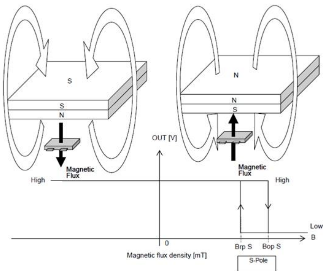
Fig 4, Magnetic Operation Characteristic of AS1510A
